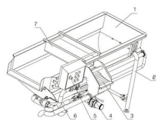
清洗槽体装置 Cleaning Tank Device
