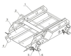
可调式振动沥水装置 Adjustable Vibrating Drain Device
